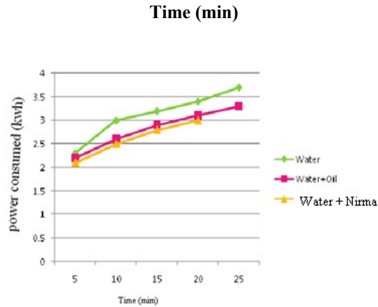
Fig 1 Performance curve for various coolant used during machining of SRB using SBDT on 1.6-meter Dia Blade Machine
