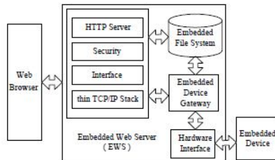
Figure 2. The EWS software architecture
