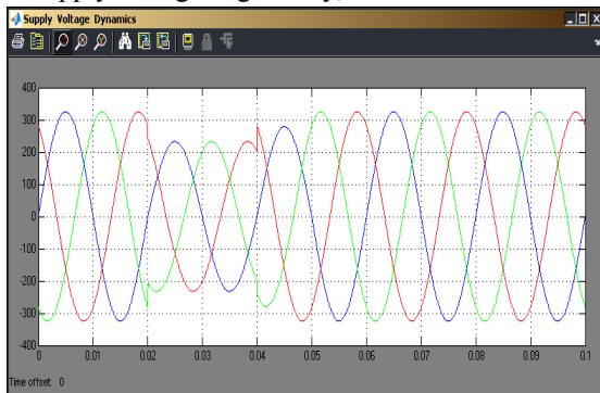
Figure 9 Supply Voltage
