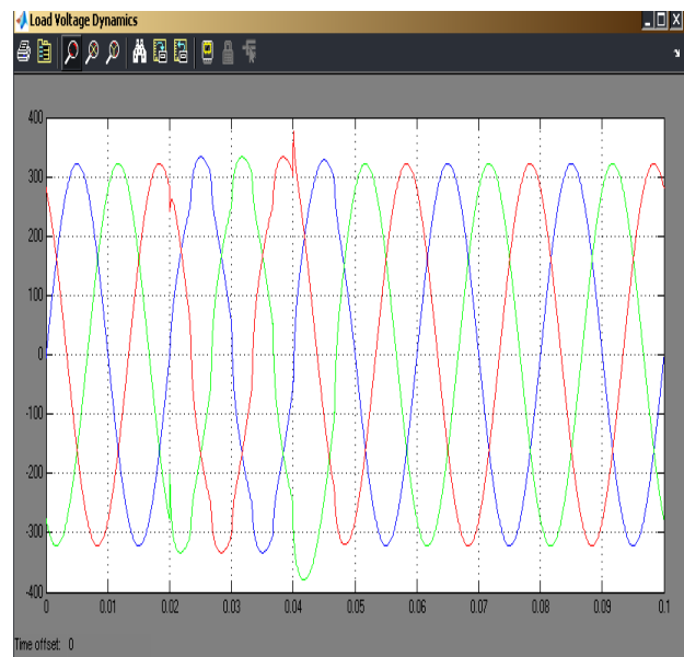
Figure 11 Load Voltage
