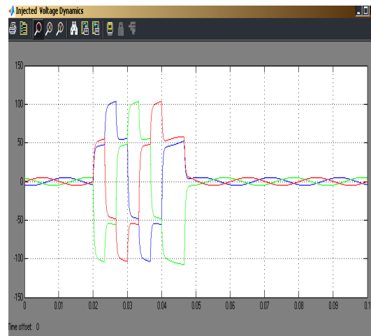
Figure 10 Injected Voltage
