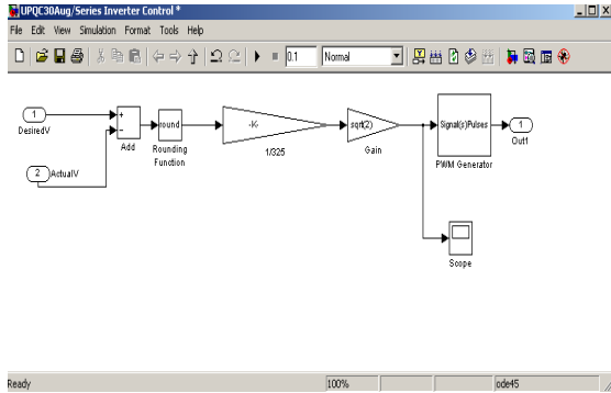
Figure 8 Series Inverter Controller.
