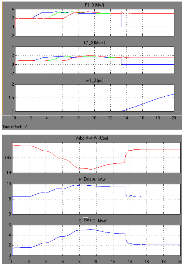
Fig.4.3. Three phase fault in wind farm and bus with out STATCOM
