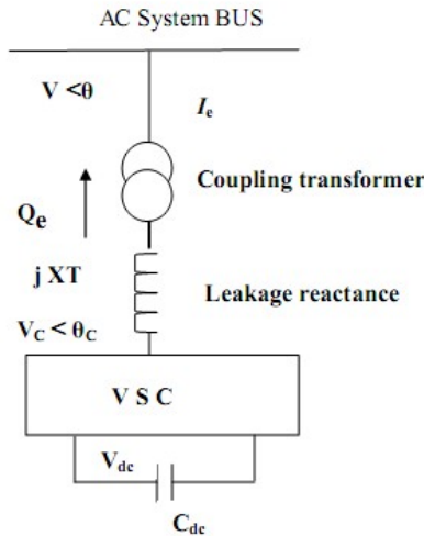
Fig. 2.1 Basic model of a STATCOM
