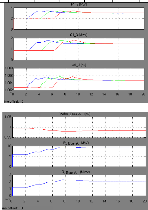
Fig.4.4. Three phase fault in wind farm and bus with STATCOM
