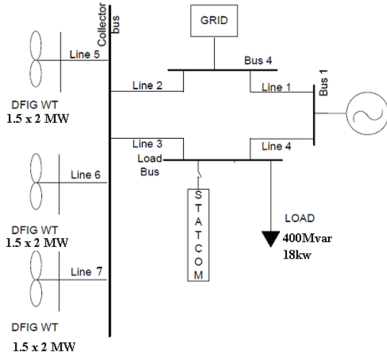
Fig. 2.3 Test Model for SIMULATION
