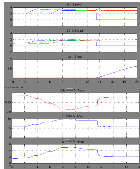
Fig.4.1. LLL fault in wind farm and bus with out STATCOM
