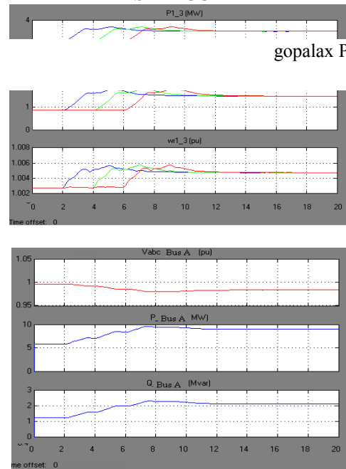
Fig.4.2. LLL fault in wind farm and bus with STATCOM
