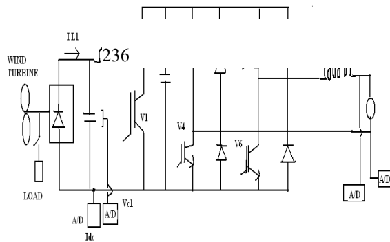
Fig.2.4 PWM circuit for control and DC-AC inverter
