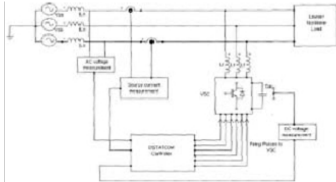
Figure2: Schematic diagram of DSTATCOM control
