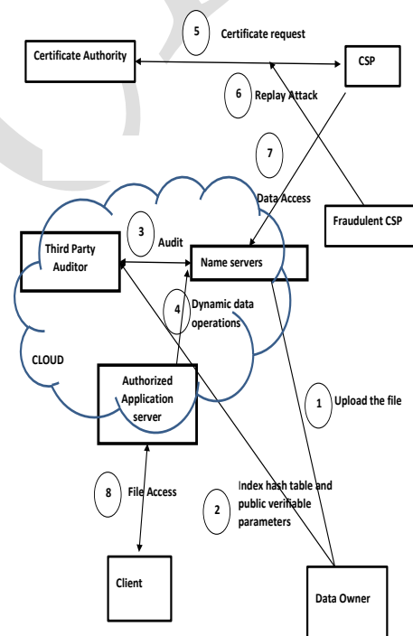
Figure 1 – Certified Secure Storage Service Architecture
